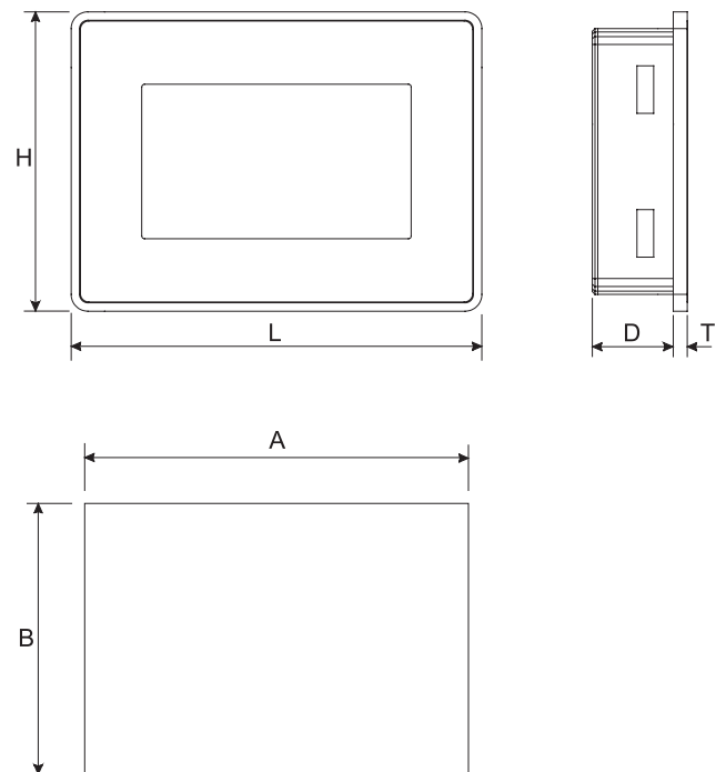
Cut-out
